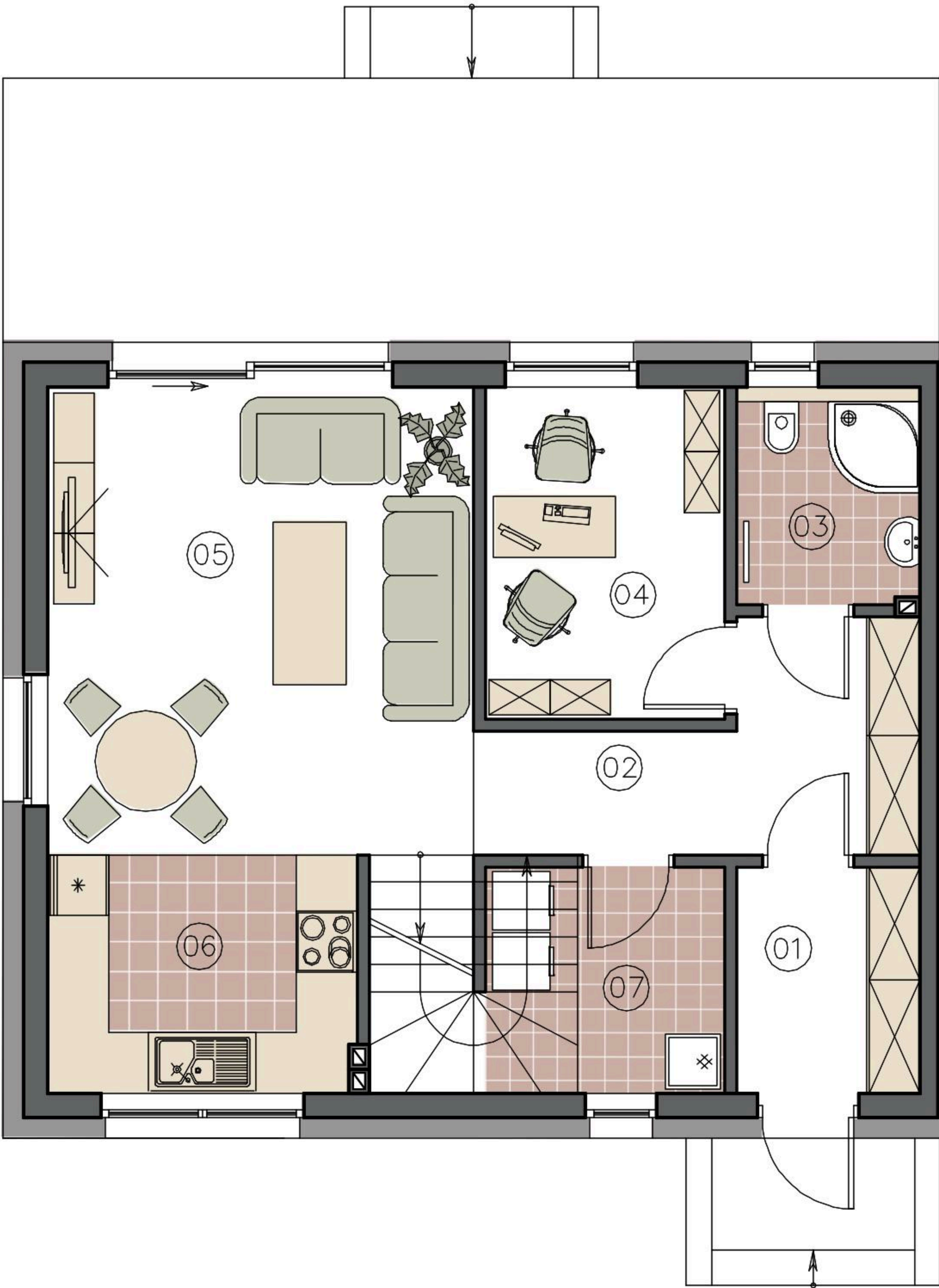
PARTER
